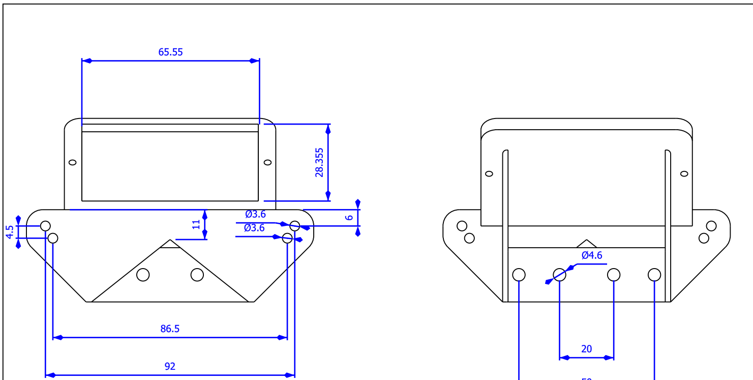
These 3.6mm holes fit for KVANT Lasers
